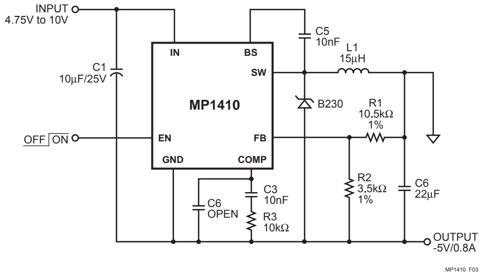
Figure 3—Application Circuit for -5V Supply
