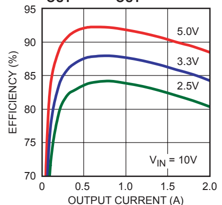
Efficiency vs I OUT and V OUT
