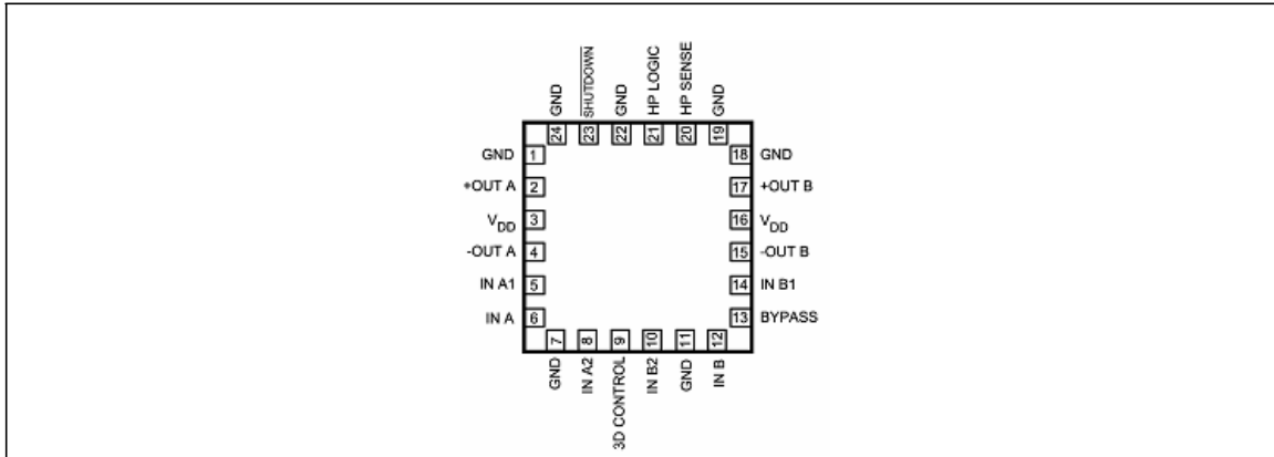
Figure 1. ft4888 Pinout Diagram
