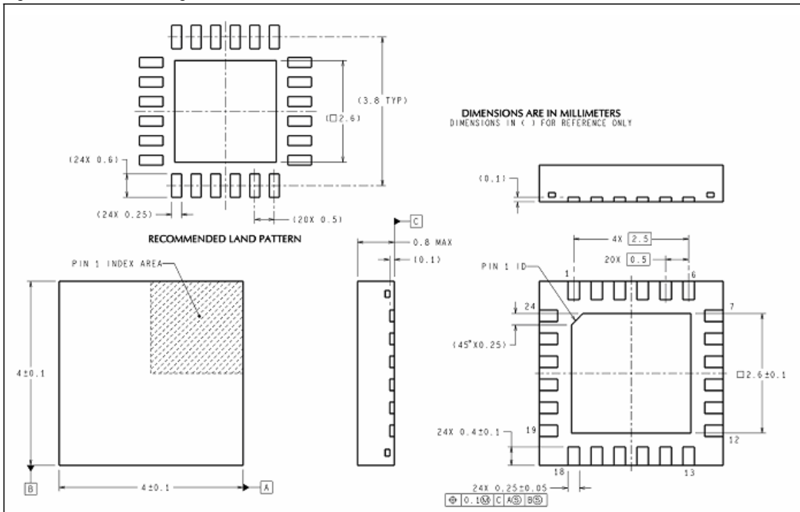
Figure 2. ft4888 Package Dimensions
