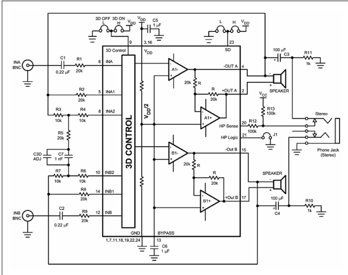
Figure 3. Typical Application Schematics
